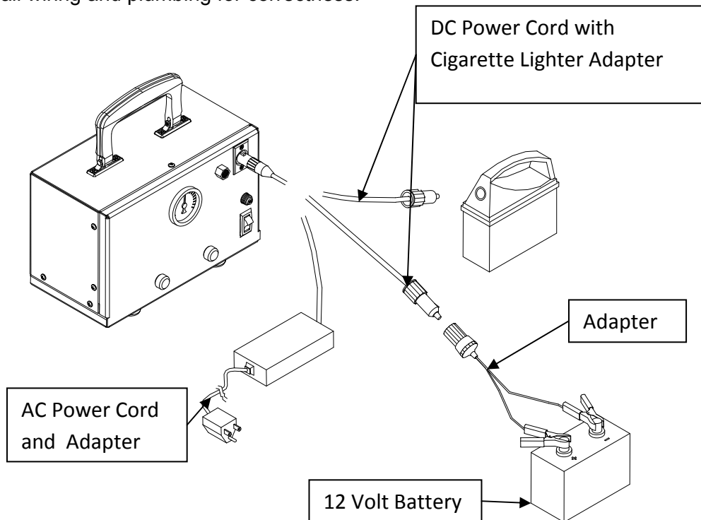
Figure 2 – Installation Diagram
